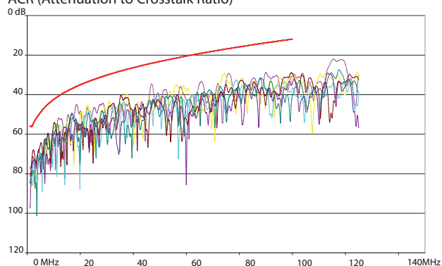
ACR (Attenuation to Crosstalk Ratio)
