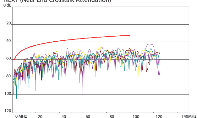
NEXT (Near End Crosstalk Attenuation)
