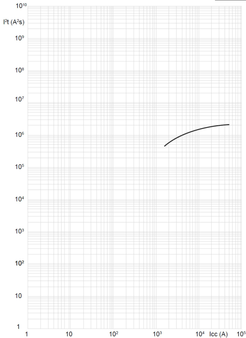
10.3 Pass-through specific energy characteristic curve
