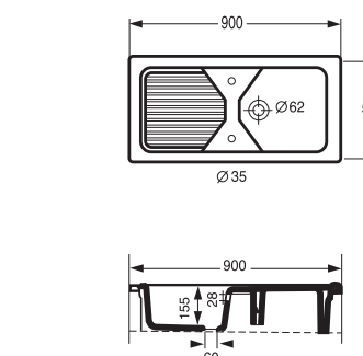
Evier de cuisine a poser 90x50cm Kitchen sink 90x50cm 32 Kg
