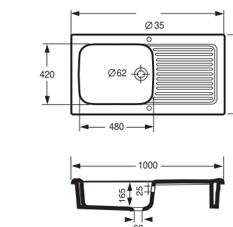
Evier de cuisine a poser 100x60cm Kitchen sink 100x60cm 36 Kg
