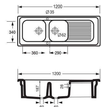
Evier de cuisine a poser 120x50cm Kitchen sink 120x50cm 48 Kg
